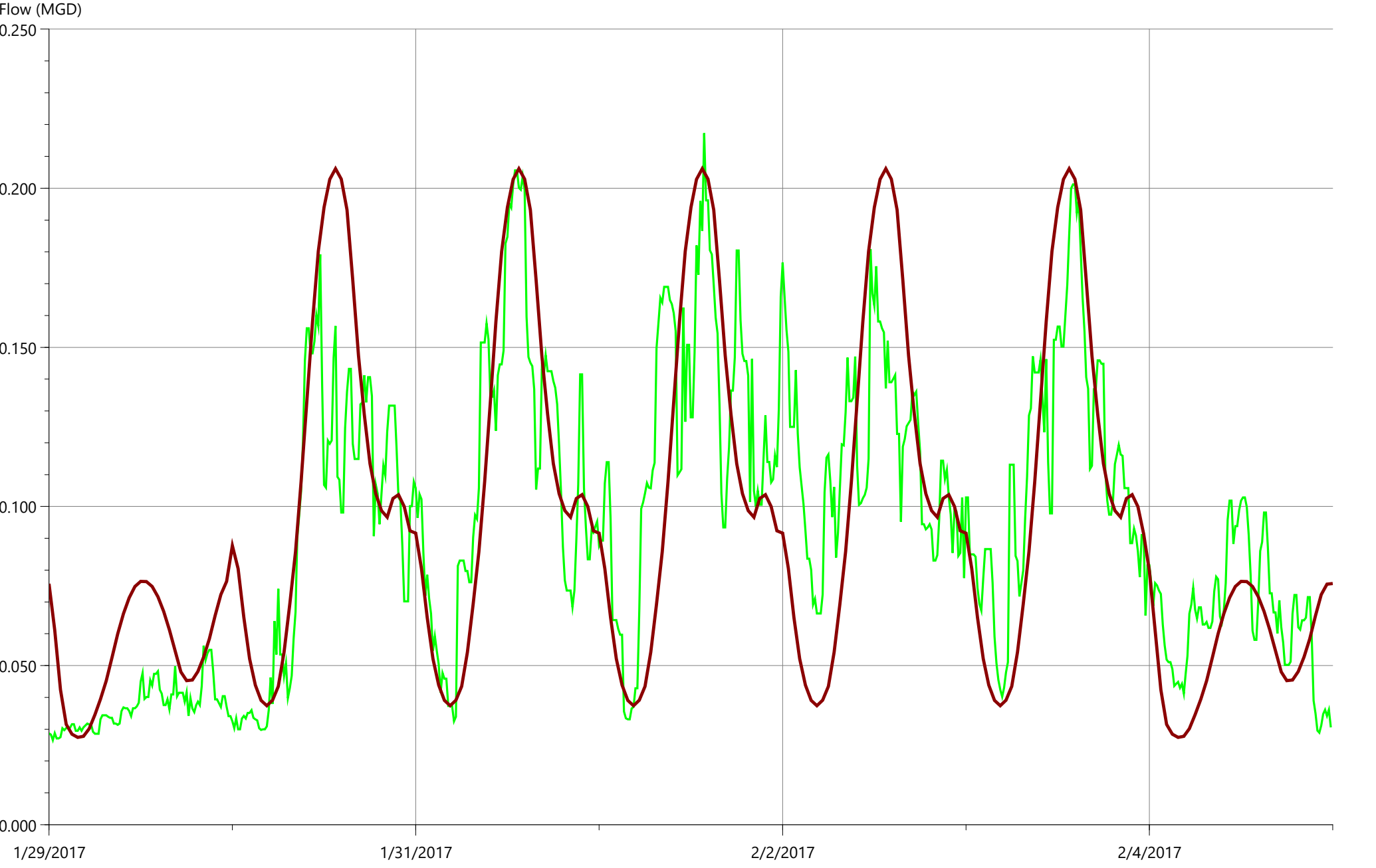
Flow Survey Location (Obs.) FM1, Model Location (Pred.) D/S D21-5042.1
