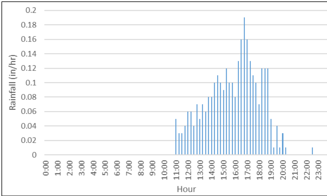
Figure 6-2: Design Storm (10-year, 12-hour)
